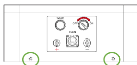
Figure 4-1 BDU right interface
