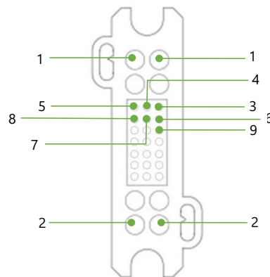
Figure 2-6 Composite Connector-Socket
