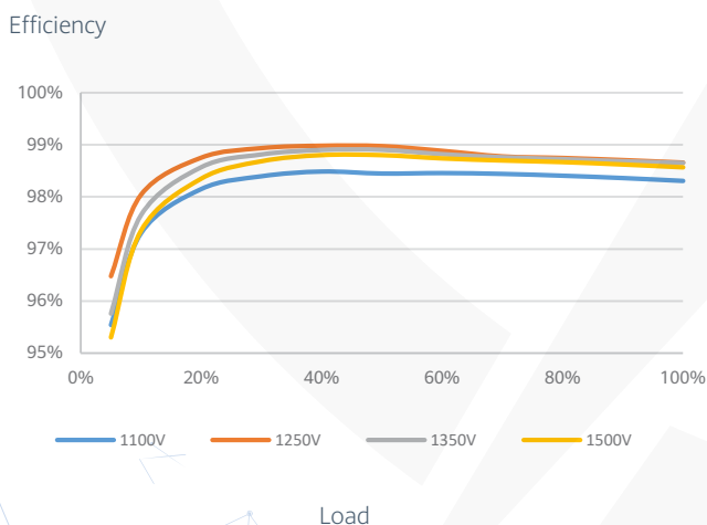
Efficiency Curve
