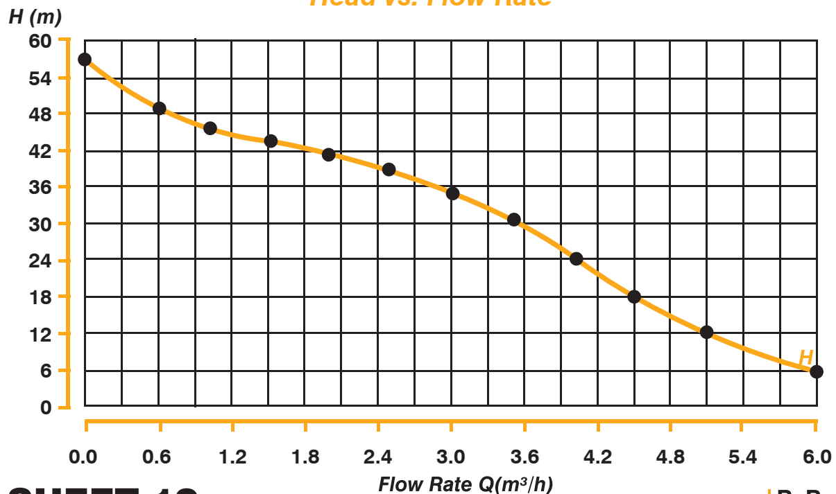
Head vs. Flow Rate
