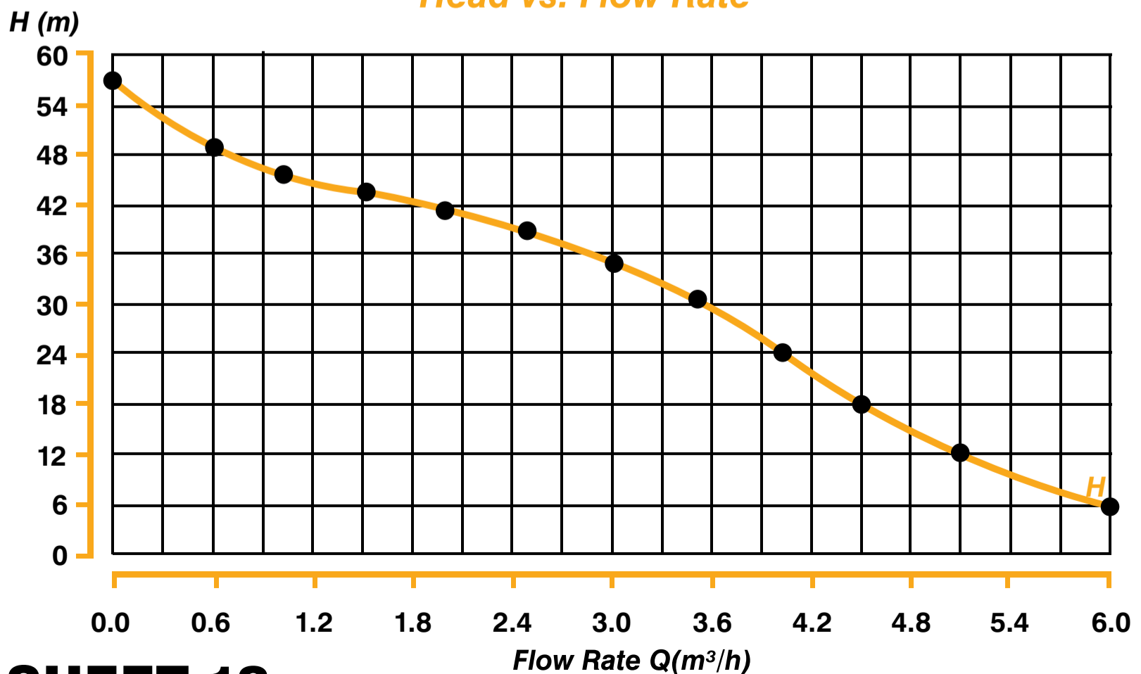
Head vs. Flow Rate
